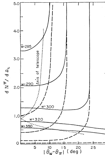
FIG. 2. Kinematics of charged pions from p+d \rightarrow \text{He}^3 + \pi^+ + \pi^- for T_p=743 MeV and a \text{He}^3 laboratory angle of 11.8 deg. The angle \theta_w is the laboratory angle of the vector sum of the momenta of the two pions, \theta_\pi is the pion laboratory angle, and dN_\pi/d\Omega is the pion laboratory cross section.
