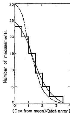
FIG. 3. Test of consistency of the measurements of the \pi - \text{He}^3 coincidence rates. The histogram shows the deviations of 76 separate measurements in terms of their statistical errors. The dashed curve is the normal distribution. The solid curve results if the errors on the measurements are increased by 25%.
